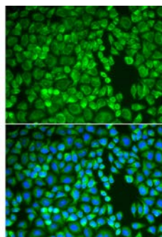
Fig. 3. Immunofluorescence analysis of A549 cells using IDE antibody. Blue: DAPI for nuclear staining.
